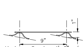
SLAB SPACER DETAIL
