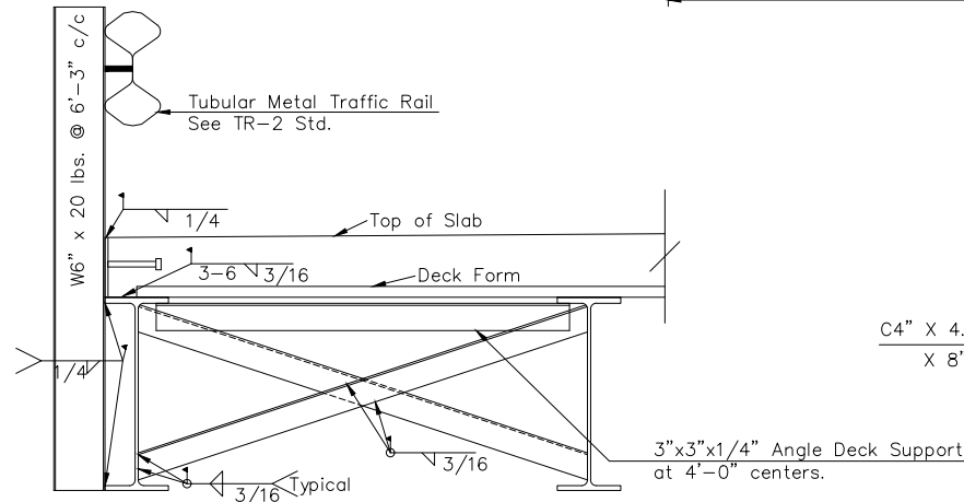
TR-2 TRAFFIC RAIL & DIAPHRAM DETAIL (Rail, Posts & all fastener hardware to be included in price bid for Handrail)
