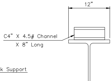
SHEAR CONNECTORS Existing Shear Connectors shall remain in place. Add additional Shear Connectors to insure a maximum row spacing of 12".
